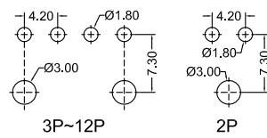
Recommended P.C.B Layout General Tolerance±0.05
