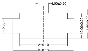
DUAL ROW RECOMMENDED RANEL CUT-OUT (DESIGNED FOR 0.80mm TO 2.00mm THICK STAMPED PANEL OR PRINTED CIRCUIT BOARD)
