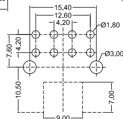
Recommended P.C.B Layout General Tolerance \pm 0.05
