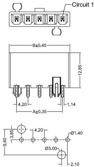
Recommended P.C.B Layout General Tolerance±0.05
