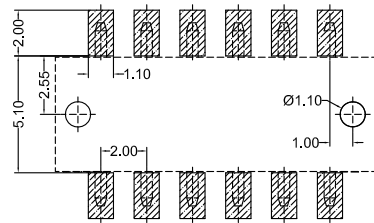
Recommended P.C.B Layout General Tolerance±0.05
