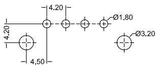
Recommended P.C.B Layout General Tolerance±0.05
