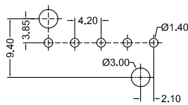
Recommended P.C.B Layout General Tolerance±0.05
