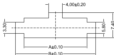
SINGLE ROW RECOMMENDED PANEL CUT-OUT (DESIGNED FOR 0.80mm TO 2.00mm THICK STAMPED PANEL OR PRINTED CIRCUIT BOARD)
