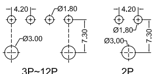
Recommended P.C.B Layout General Tolerance±0.05
