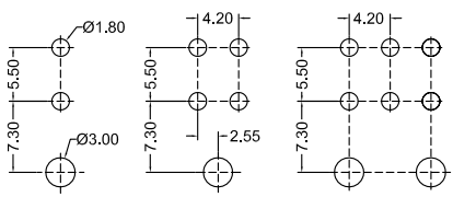
Recommended P.C.B Layout General Tolerance±0.05
