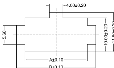
DUAL ROW RECOMMENDED RANEL CUT-OUT (DESIGNED FOR 0.80mm TO 2.00mm THICK STAMPED PANEL OR PRINTED CIRCUIT BOARD)
